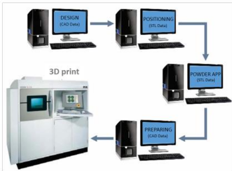
Figure 9. Schematic representation of the manufacturing of a frame using the SLM technology [20]
