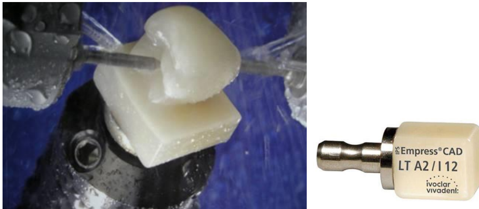
Figure 7. Left – the action of milling a ceramic crown in an in-office CAD/CAM machine; right – a ceramic block from which the ceramic crown is milled
