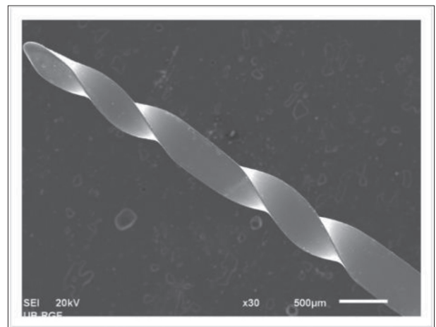
Figure 6. Spin echo image BioRaCe instrument no. 4 without incorporation and corrosion (30 ×)
