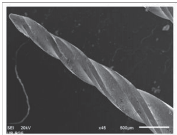
Figure 4. Spin echo image K3 instrument (25–0.08), second experimental group (corrosion on the apical third) (45 ×)
