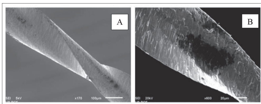
Figure 1. Spin echo image of the new Mtwo instrument (10/0.4): A – surface of the middle third on which the presence of corrosion is observed (170 ×); B – detail from the previous image at higher magnification (600 ×)
